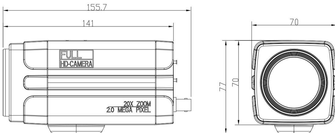
Pic 2.1.1 Camera dimension
