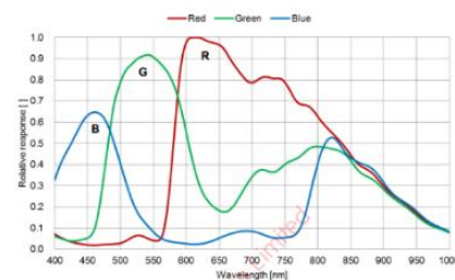
MV-CH089-10GC Quantum Efficiency
