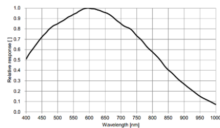
MV-CH089-10GM Quantum Efficiency
