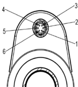
Pinning Hirose connector HR10G-7R-6PB(73)
