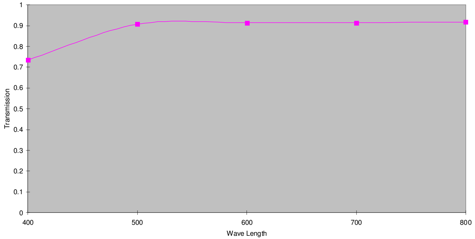
LM28CLS Transmission
