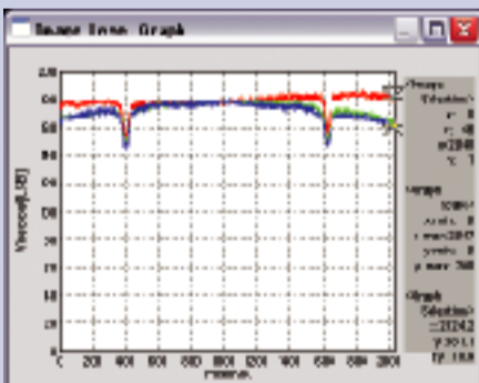
Standard Lens
