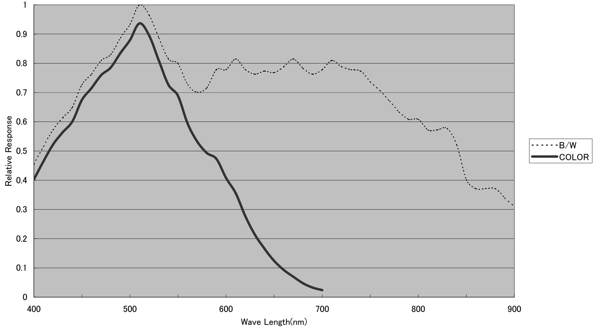
ISD-A15TDN, ISD-A35 Spectral Response
