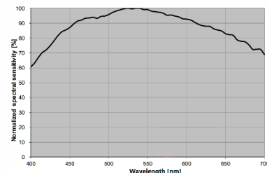
MV-CH1510-10XM-M72-NF
