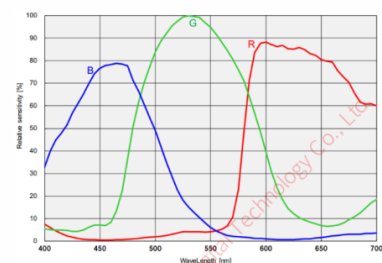
MV-CH1510-10XC-M72-NF
