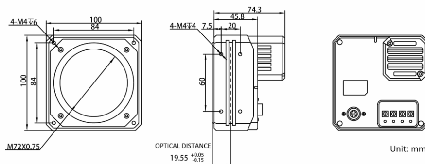
MV-CH1510-10XC-M72-NF
