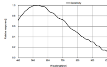
MV-CE120-10GM Quantum Efficiency
