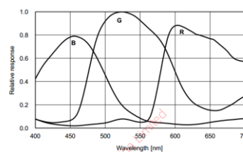
MV-CE120-10GC Quantum Efficiency
