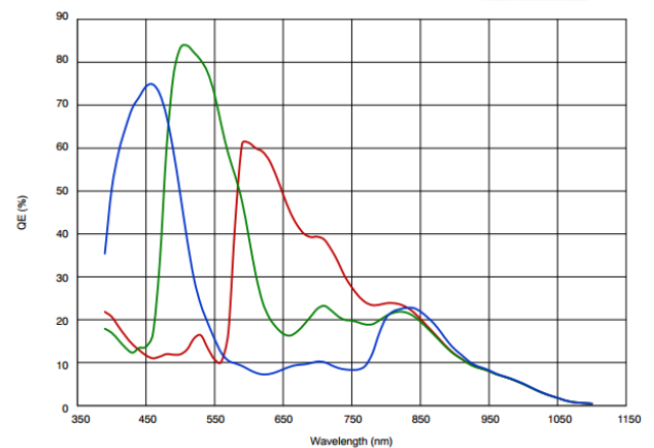
MV-CE050-30UC Quantum Efficiency
